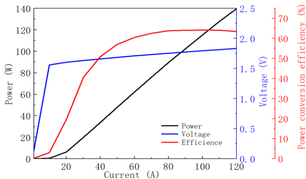
Power-Current-Voltage-Efficiency
